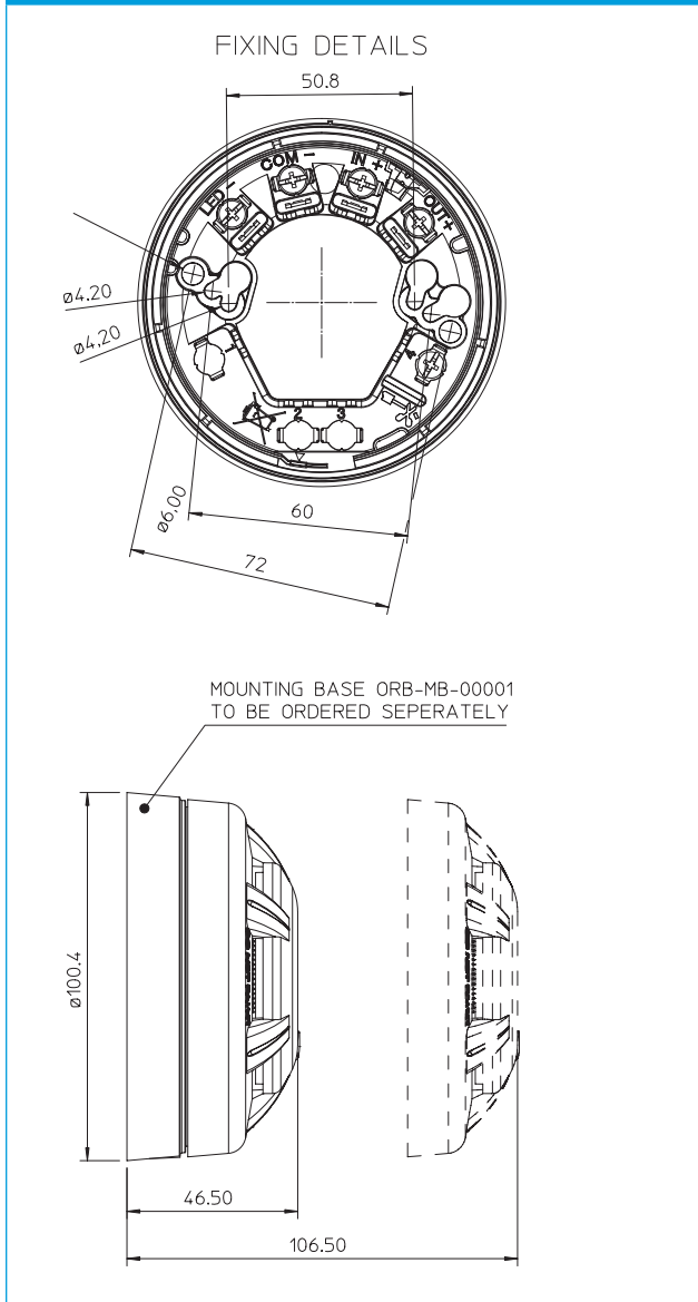
Orbis Optical Smoke Detector dimensional drawing
